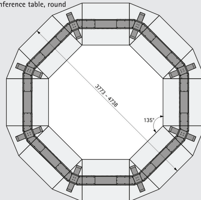
Conference table, round
