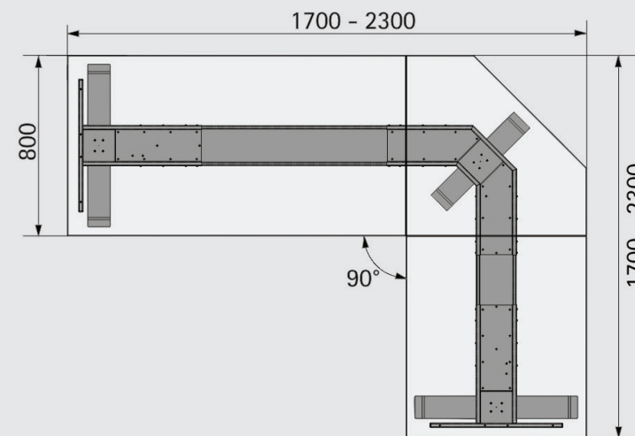
90° angle desk support
