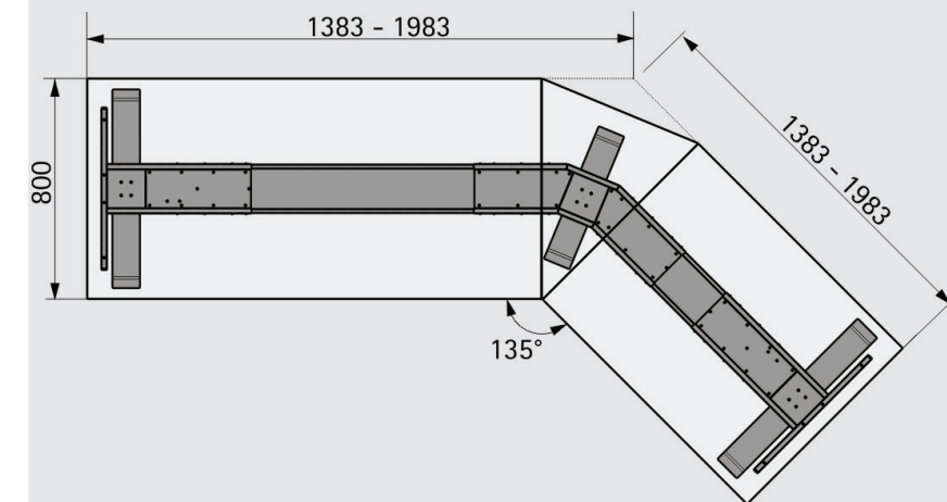
135° angle desk support
