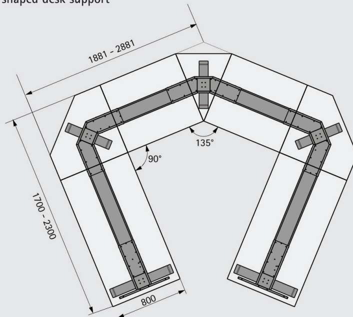
U shaped desk support
